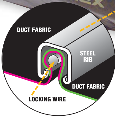
Sectional view of steel rib and duct construction
